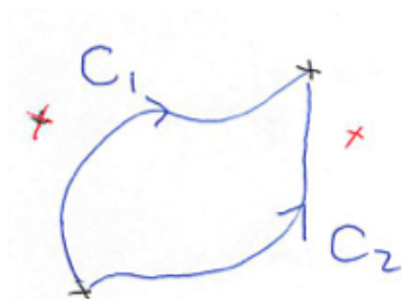
図 11: \int_{C_1} f(z) dz = \int_{C_2} f(z) dz
